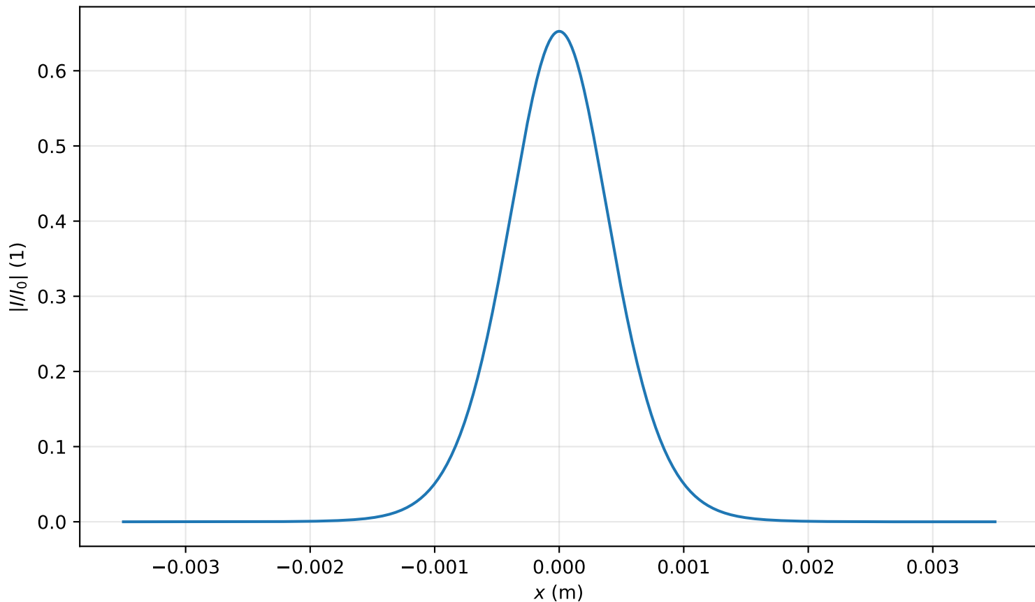
Intensity profile I(x, y = 0, z = 2.627m)/I_0 , P_{in}=0.5P_{cr} , artificial time
